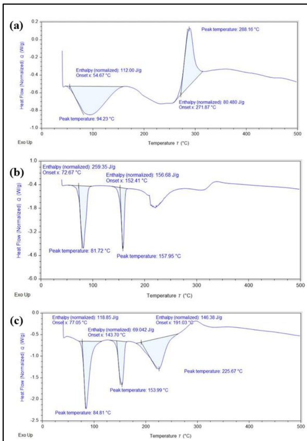
Figure 14: DSC Thermogram of (a) Liposome, (b) CoQ10 API, and (c) Liposomal CoQ10
