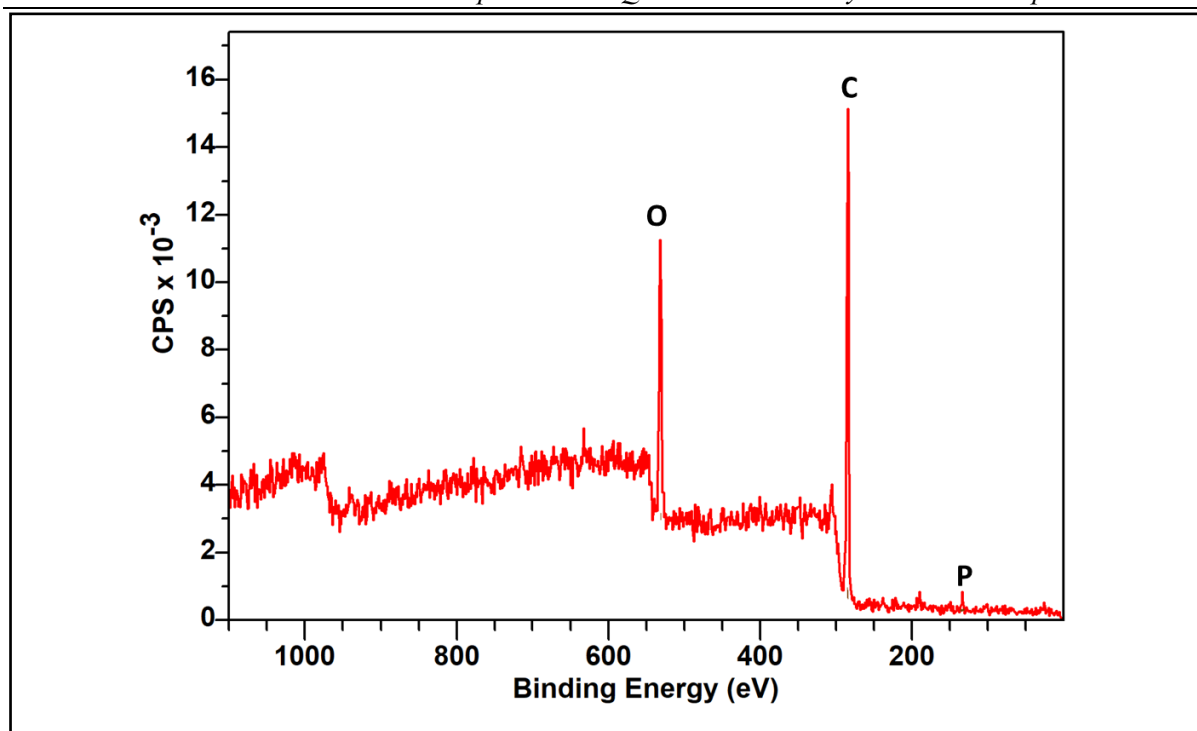
Figure 5: XPS spectrum representing different elements present in the Liposome
