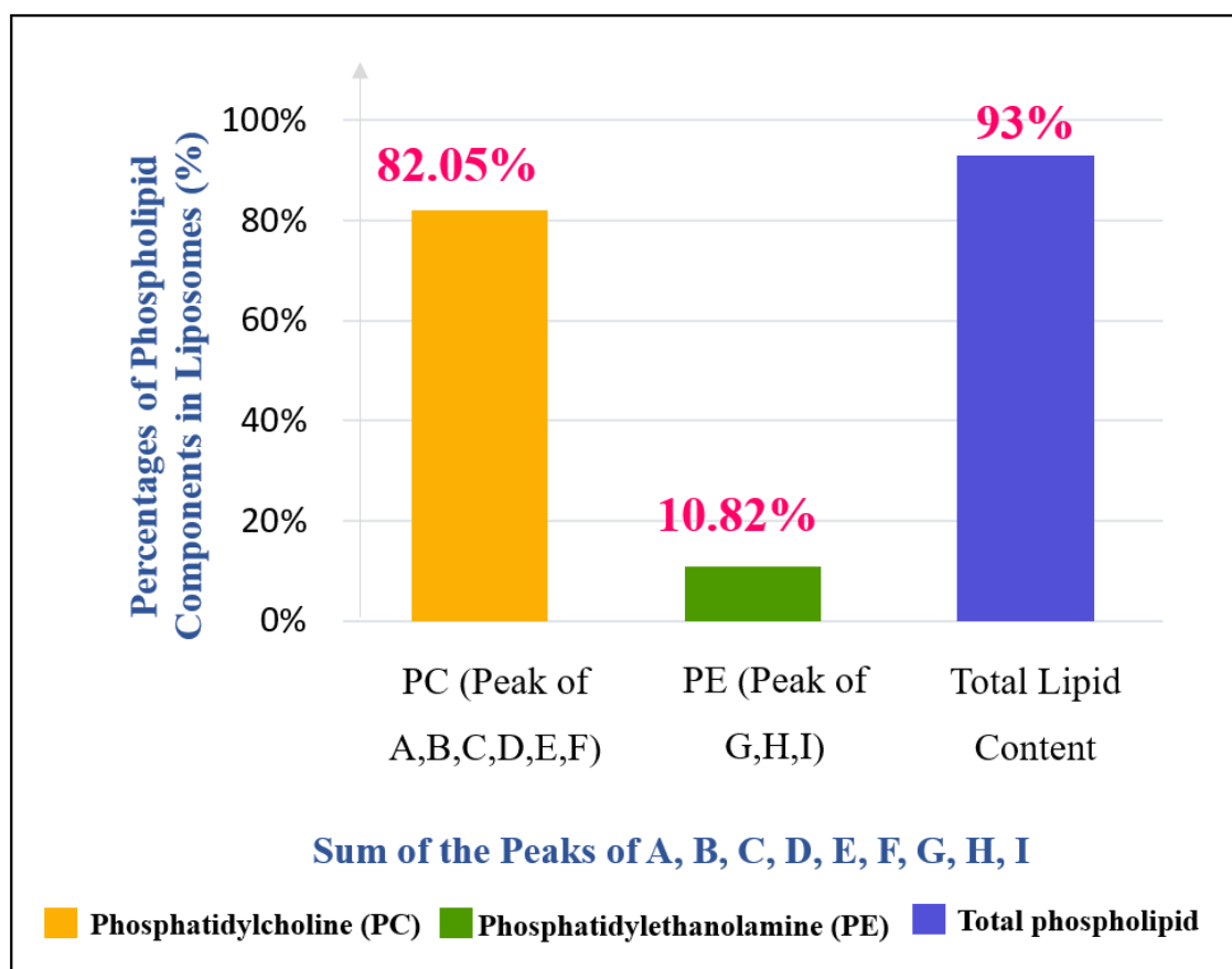
Figure 4: Chart showing composition of Liposomes with 82.05% PC and 10.82% of PE resulting in 93% total phospholipid content
