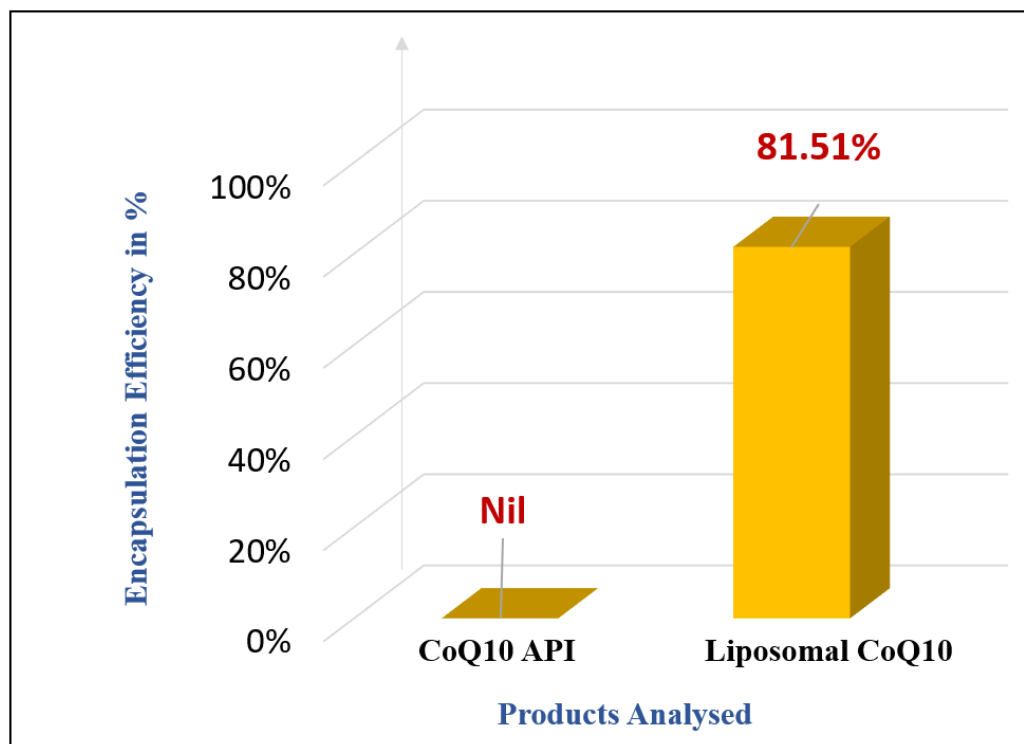
Figure 7: Encapsulation Efficiency determined via validated UV-Vis Spectrophotometry data
